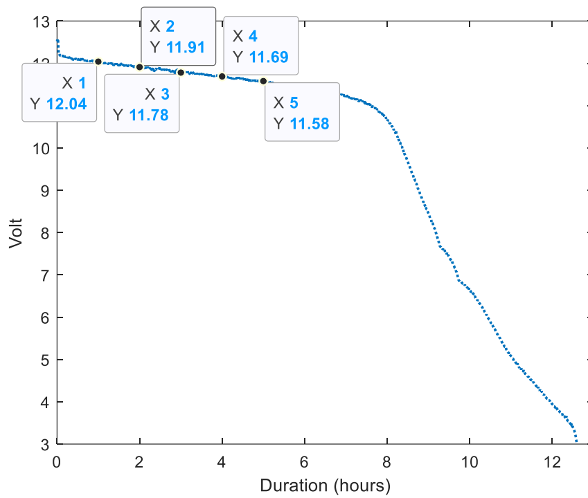
Figure B1. Five data points' collection for ANFIS testing. This data is from the discharge experiment for a 130 Watts load.
