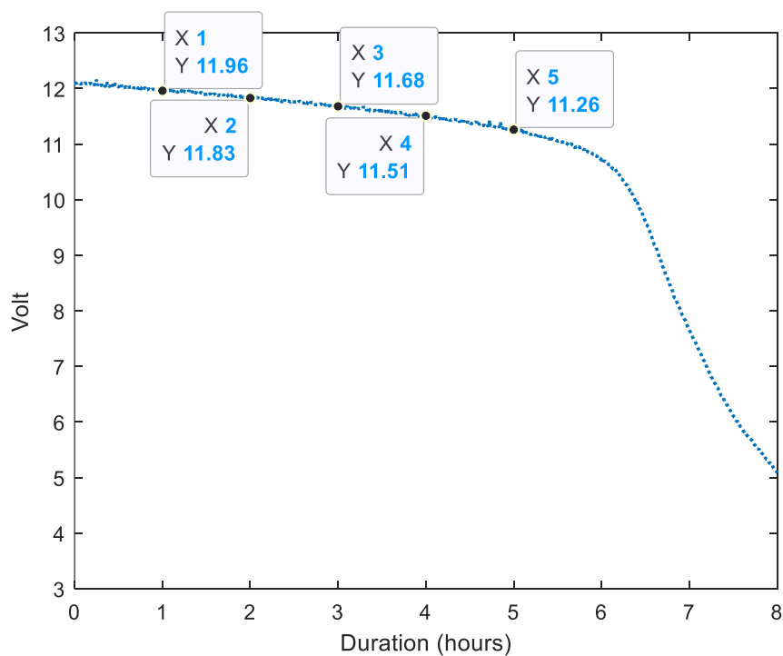
Figure B2. Five data points' collection for ANFIS testing. This data is from the discharge experiment for a 180 Watts load.
