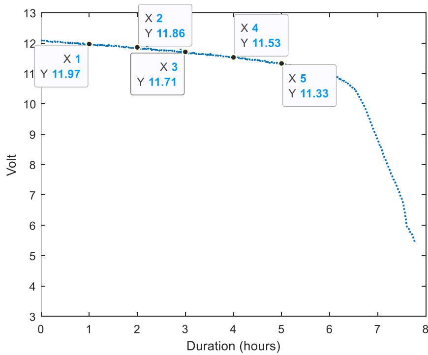
Figure A2. Five data points' collection for ANFIS training. This data is from the discharge experiment for a 180 Watts load.
