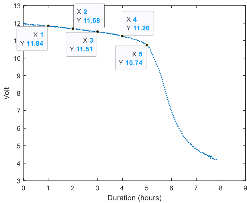
Figure B3. Five data points' collection for ANFIS testing. This data is from the discharge experiment for a 200 Watts load.
