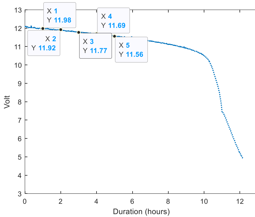
Figure A1. Five data points' collection for ANFIS training. This data is from the discharge experiment for a 130 Watts load.
