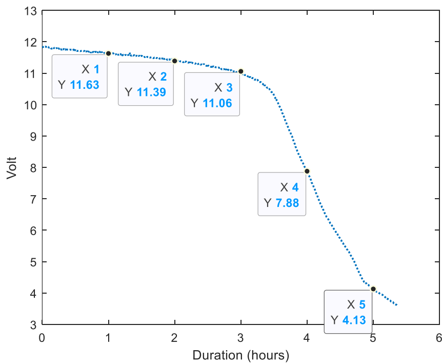
Figure B4. Five data points' collection for ANFIS testing. This data is from the discharge experiment for a 220 Watts load.
