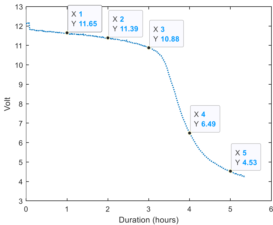
Figure A4. Five data points' collection for ANFIS training. This data is from the discharge experiment for a 220 Watts load.
