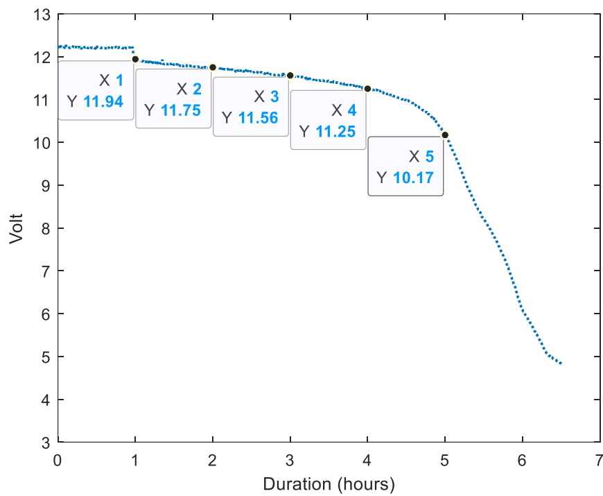
Figure A3. Five data points' collection for ANFIS training. This data is from the discharge experiment for a 200 Watts load.
